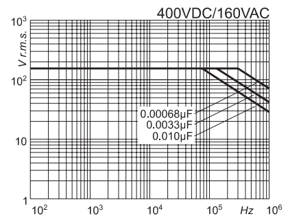
Permissible AC voltage versus frequency (sinusoidal waveform) for ΔT=+10°C Referred to the largest length execution among available ones
